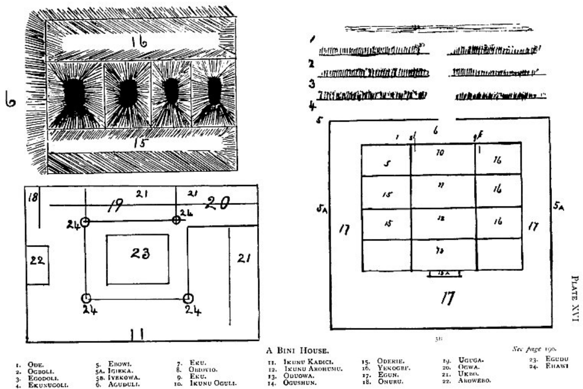
A BINI HOUSE (Pl. XVI)
